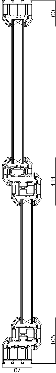
Section A - A
